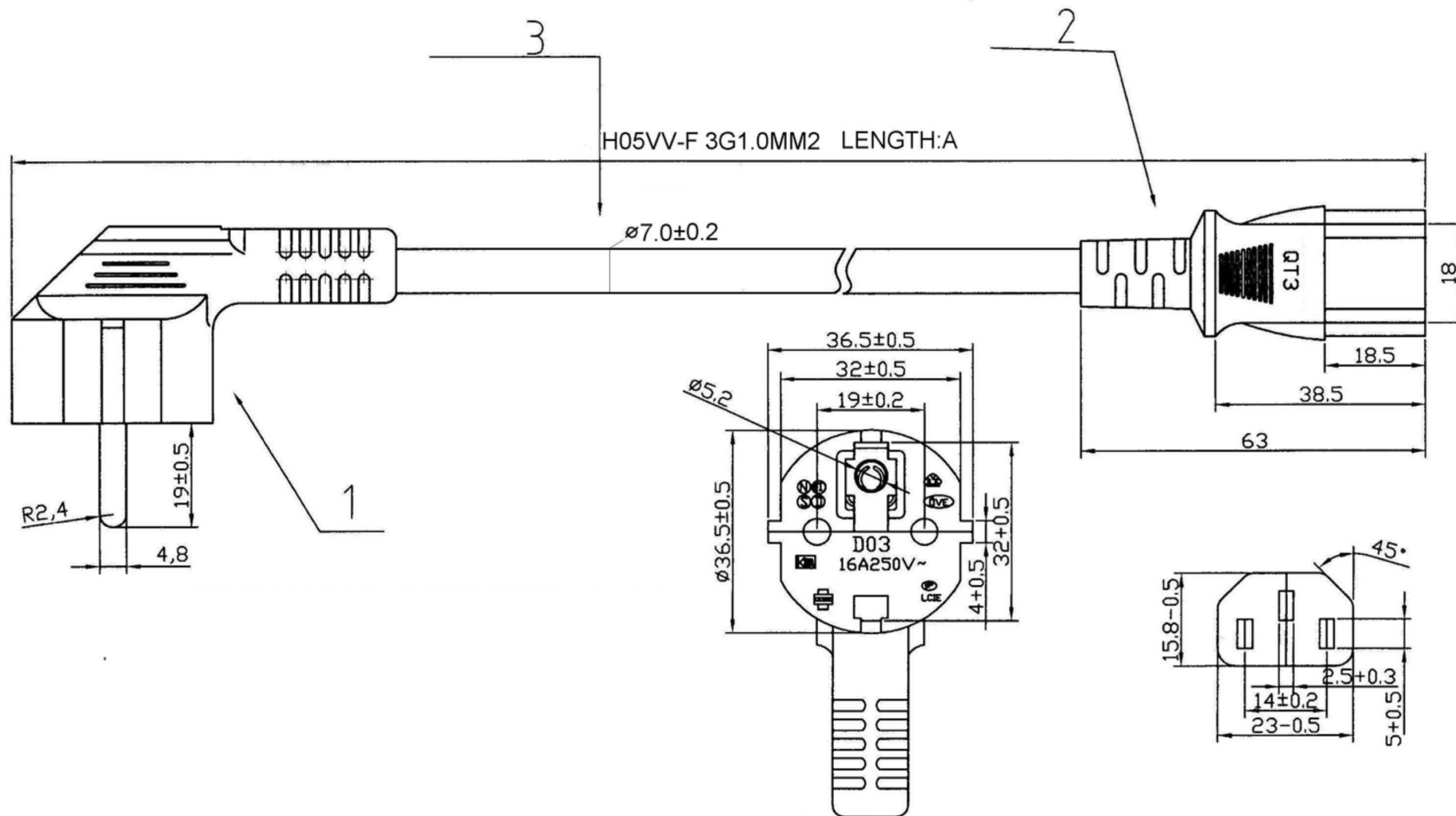
Power cord, CEE7/7 90° to C13, black, 1,0mm 2
